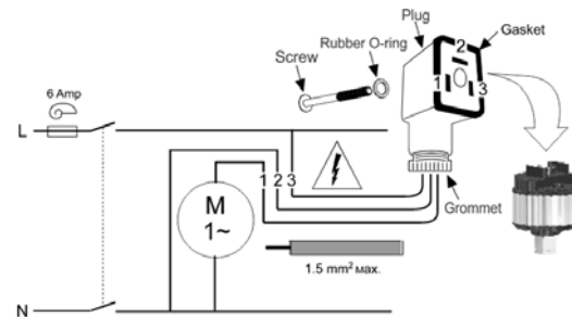
Figure 5: Wiring Details
